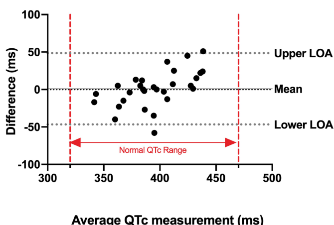
Figure 2. Bland–Altman plot comparing QTc intervals in the CardioSecur ECG (cECG) and nECG ( n=31 ). Variability is consistent and the mean difference (bias) is close to zero. One criticism would be that the 95% limits of agreement (LOAs) are marginally wide for QTc measurements.
